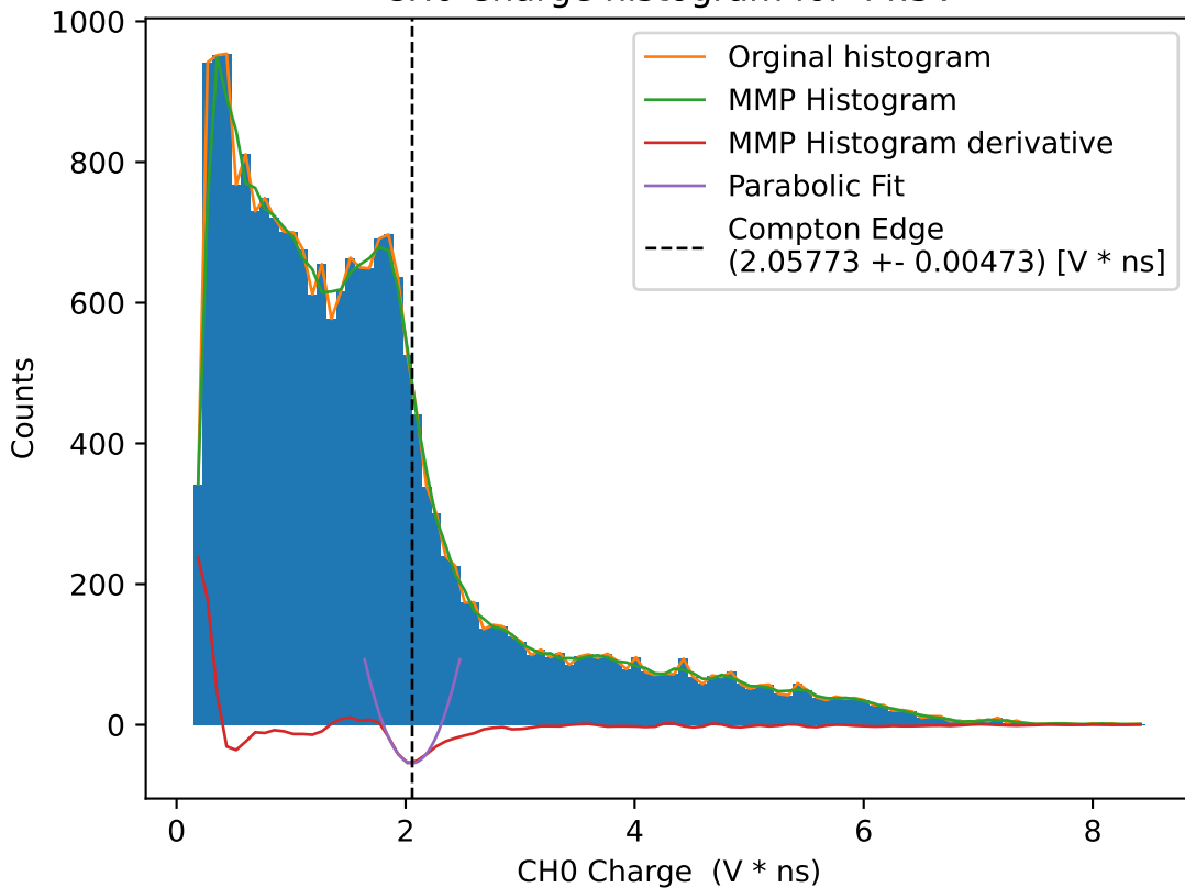
CH0 Charge histogram for 44.5V
