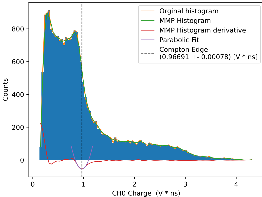
CH0 Charge histogram for 42.0V
