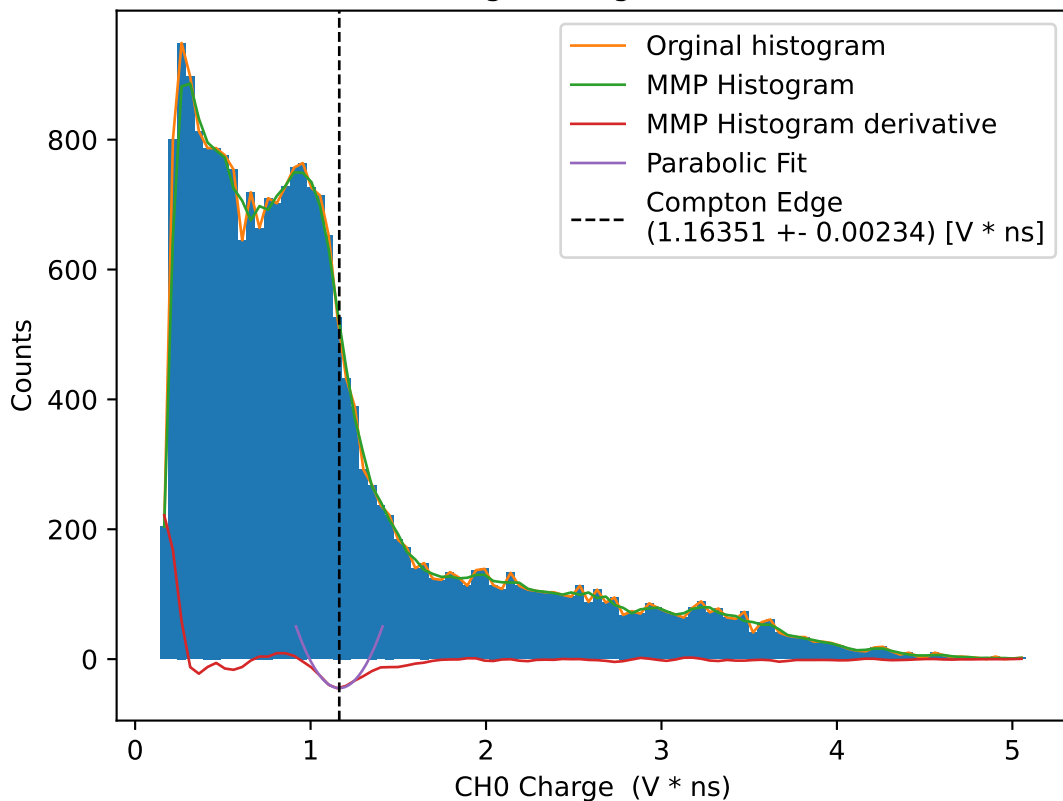
CH0 Charge histogram for 42.5V
