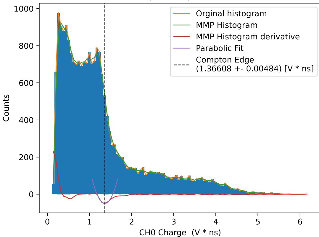
CH0 Charge histogram for 43.0V
