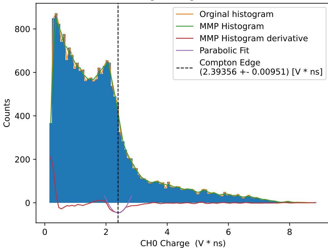
CH0 Charge histogram for 45.0V
