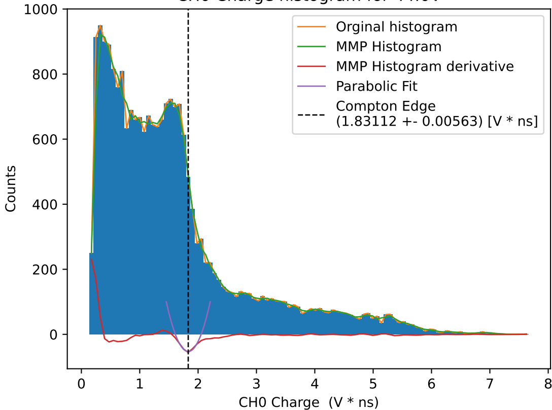
CH0 Charge histogram for 44.0V
