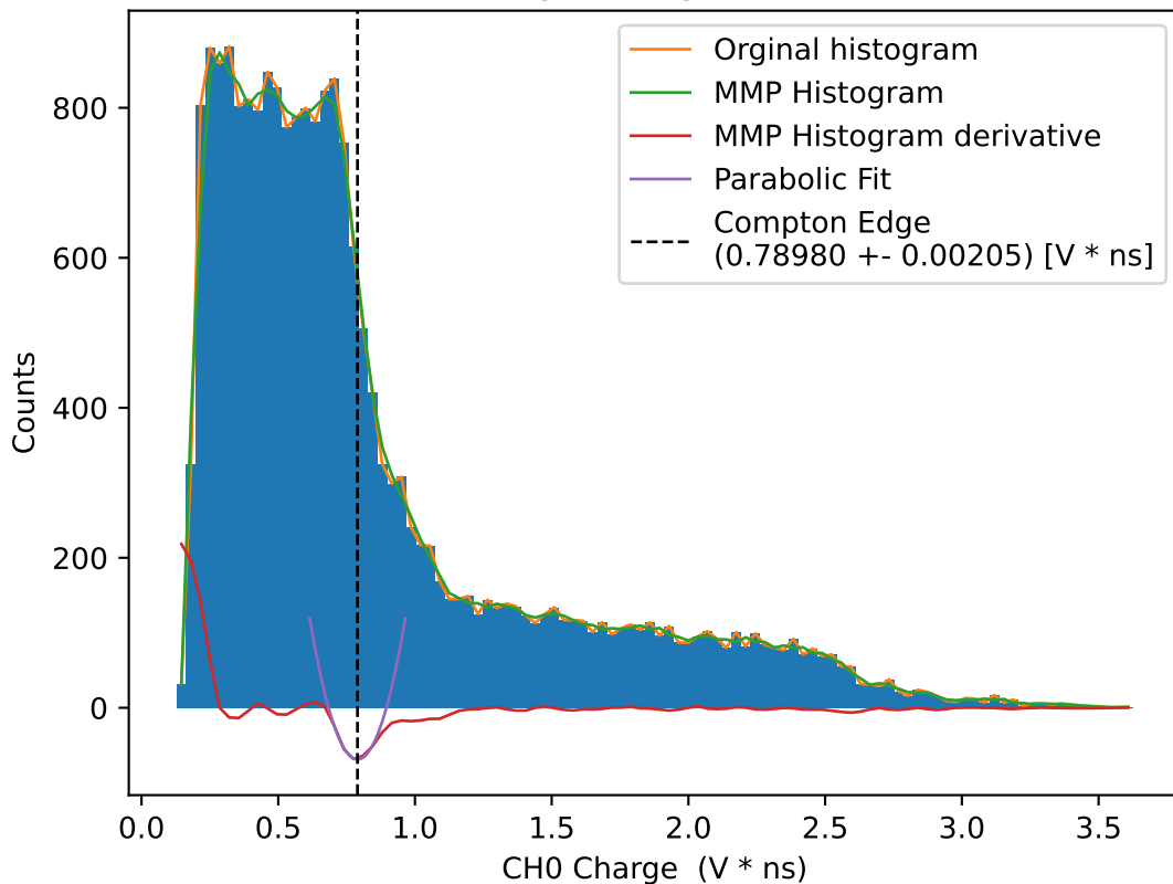
CH0 Charge histogram for 41.5V
