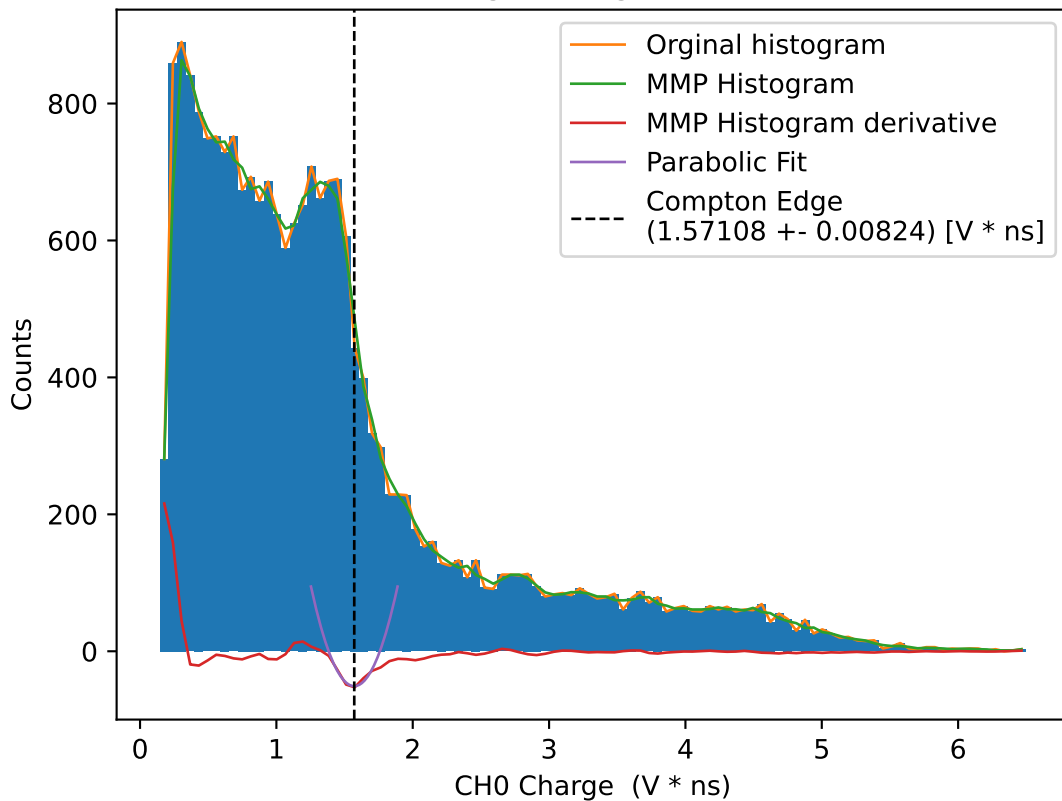
CH0 Charge histogram for 43.5V
