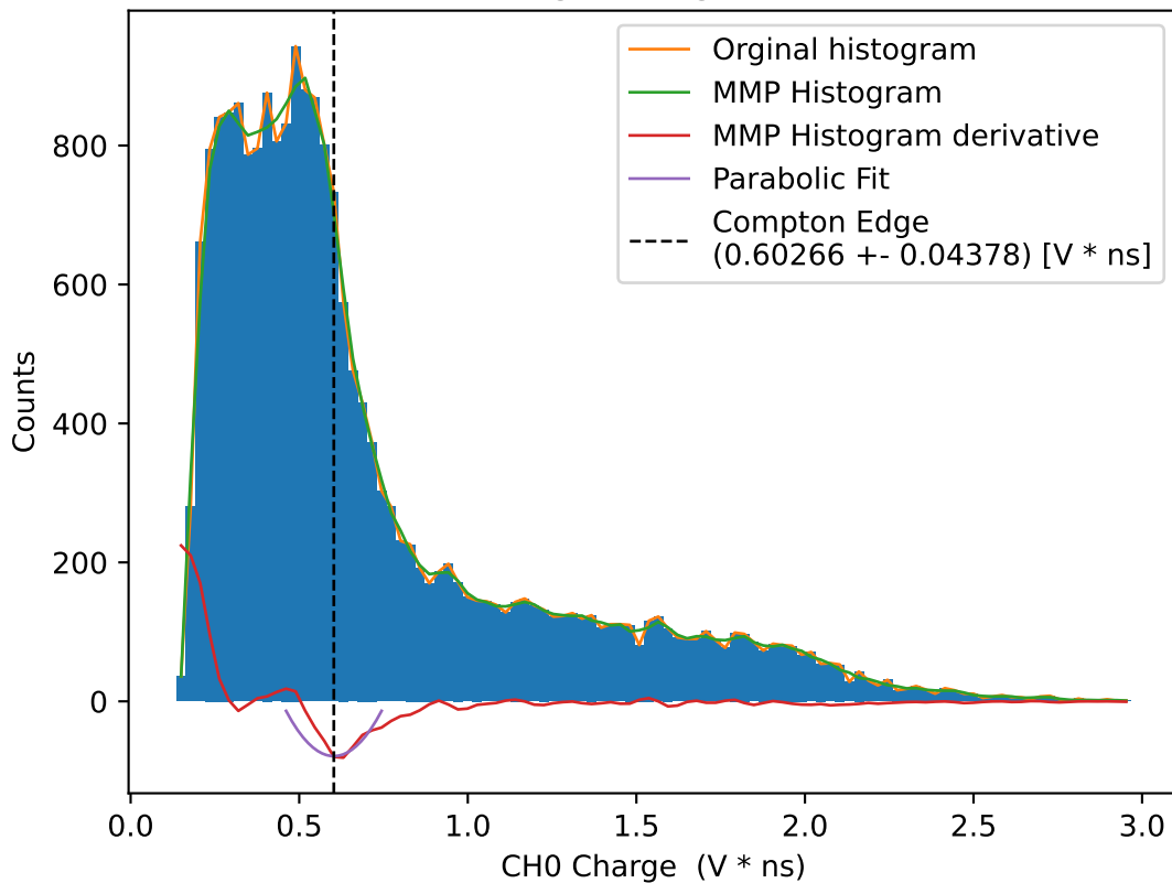
CH0 Charge histogram for 41V
